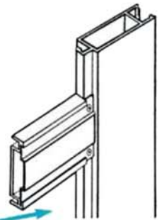
Brace Bar detail
